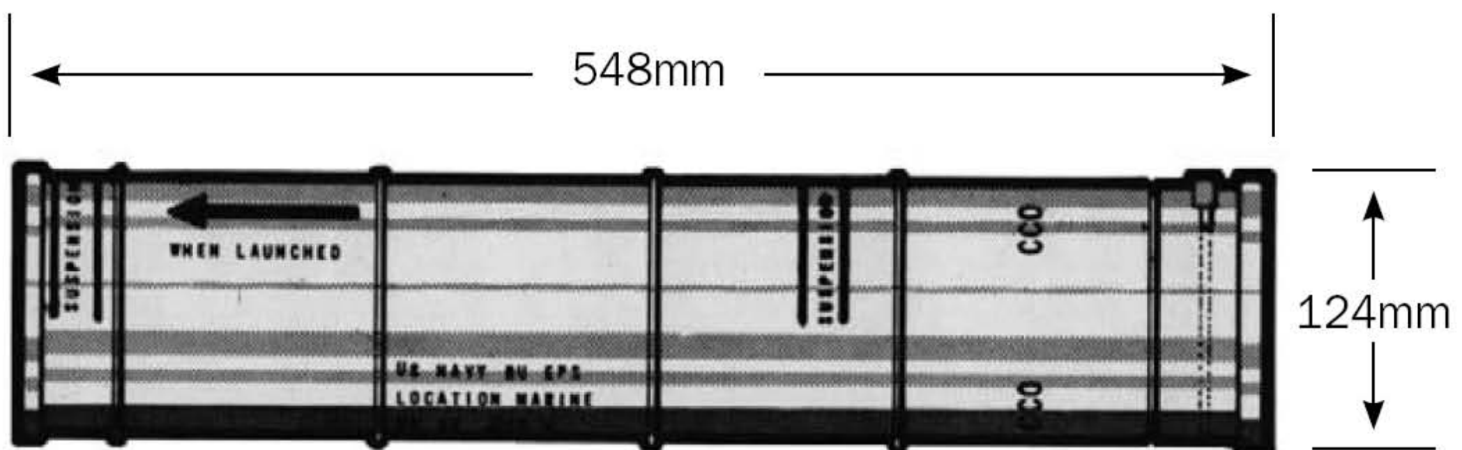
MK58 MARINE MARKER
